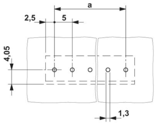
Drilling diagram
